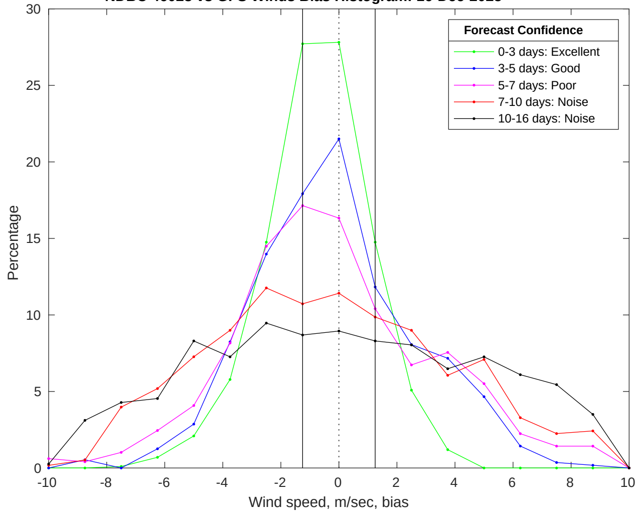
NDBC 46028 vs GFS Winds Bias Histogram: 16-Dec-2025
