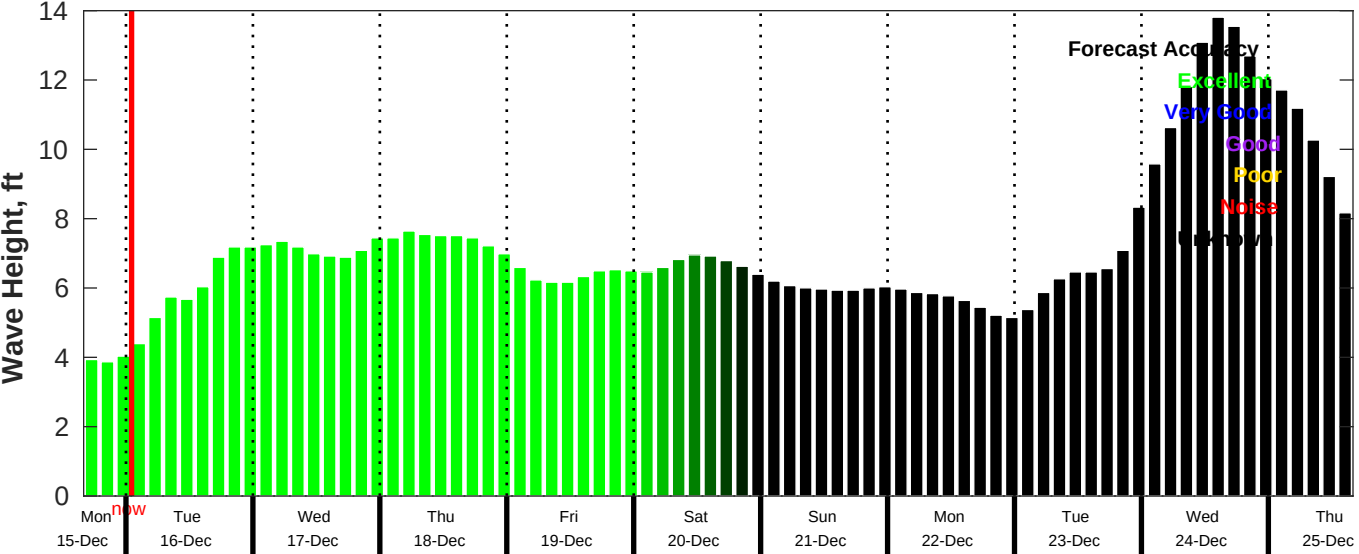
CMEMS Wave Forecast for NDBC 46028 from 15-Dec-2025 16:00:00 to 25-Dec-2025 16:00:00
