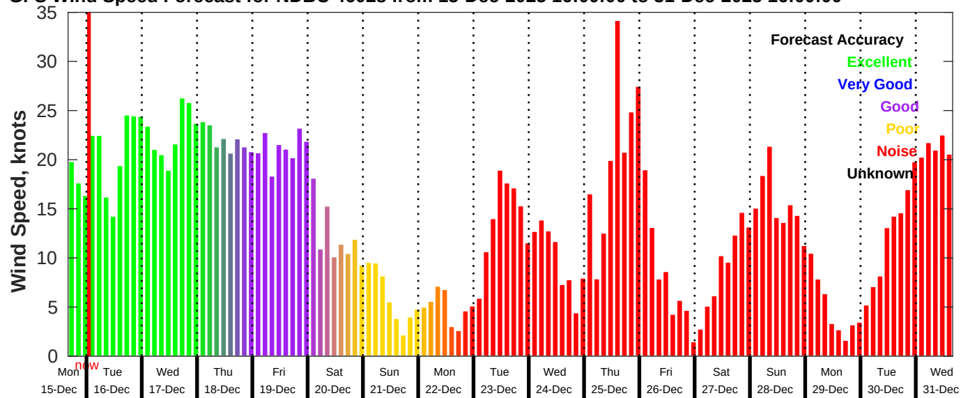
GFS Wind Speed Forecast for NDBC 46028 from 15-Dec-2025 16:00:00 to 31-Dec-2025 16:00:00
