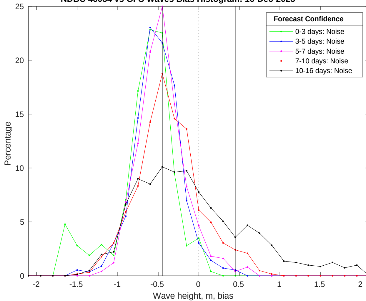
NDBC 46054 vs GFS Waves Bias Histogram: 16-Dec-2025
