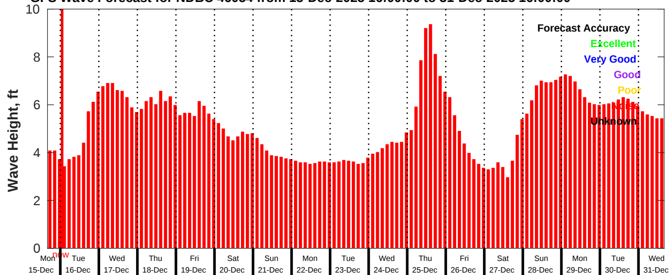
GFS Wave Forecast for NDBC 46054 from 15-Dec-2025 16:00:00 to 31-Dec-2025 16:00:00
