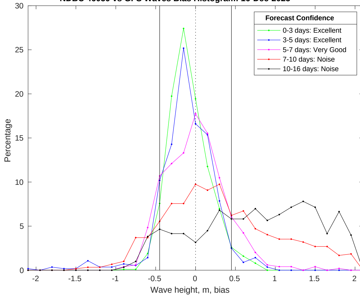
NDBC 46059 vs GFS Waves Bias Histogram: 16-Dec-2025
