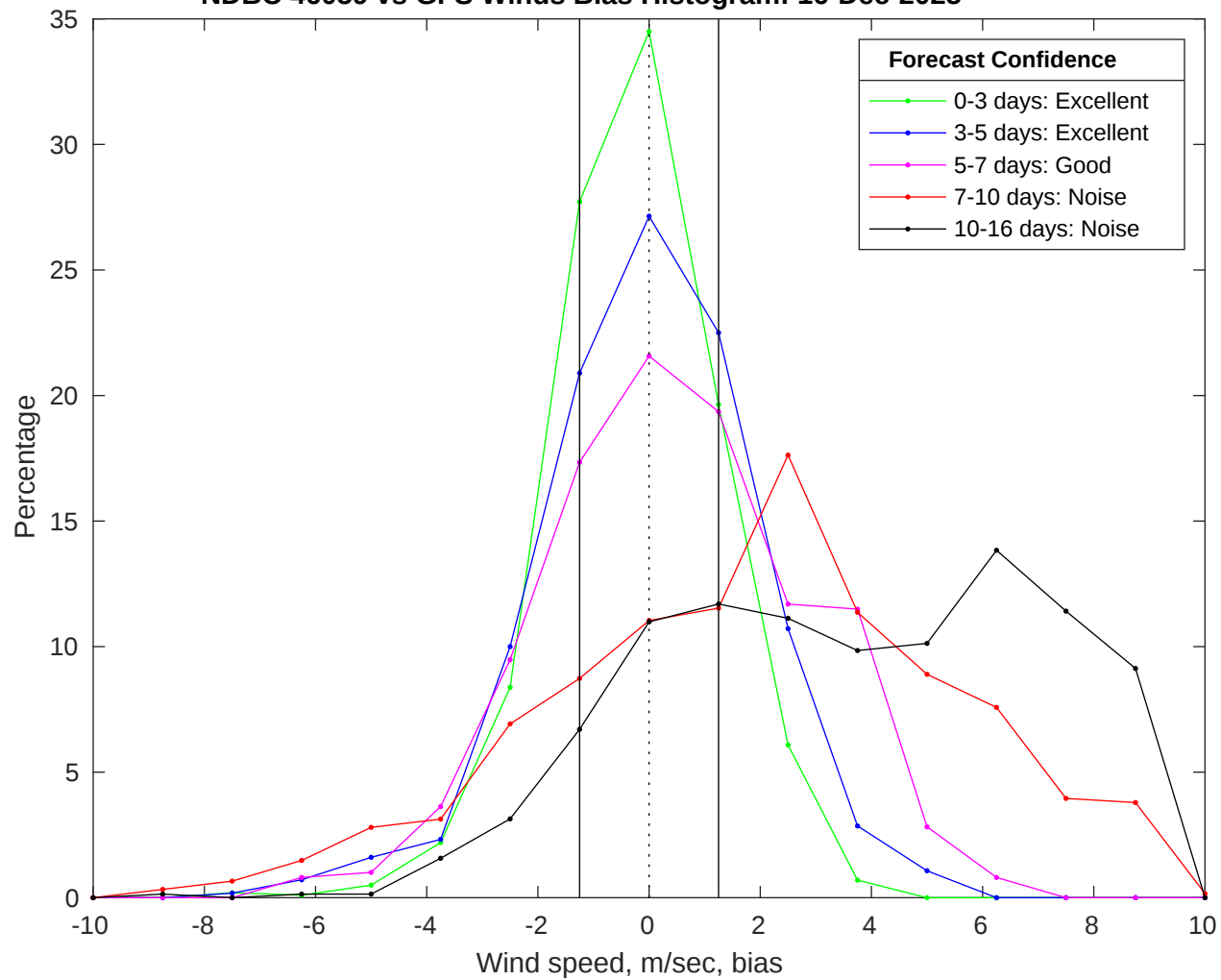
NDBC 46059 vs GFS Winds Bias Histogram: 16-Dec-2025
