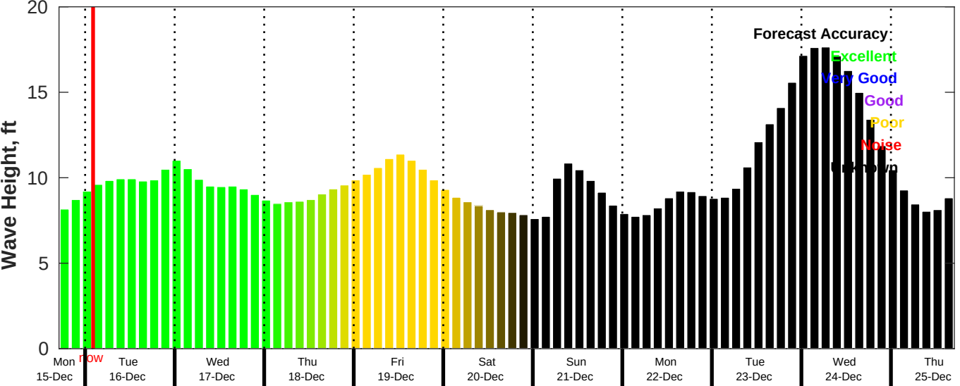
CMEMS Wave Forecast for NDBC 46059 from 15-Dec-2025 17:00:00 to 25-Dec-2025 17:00:00
