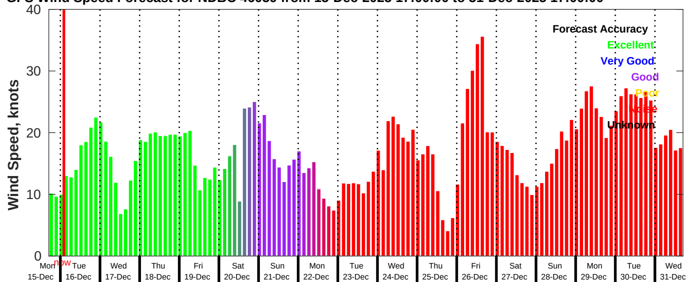
GFS Wind Speed Forecast for NDBC 46059 from 15-Dec-2025 17:00:00 to 31-Dec-2025 17:00:00
