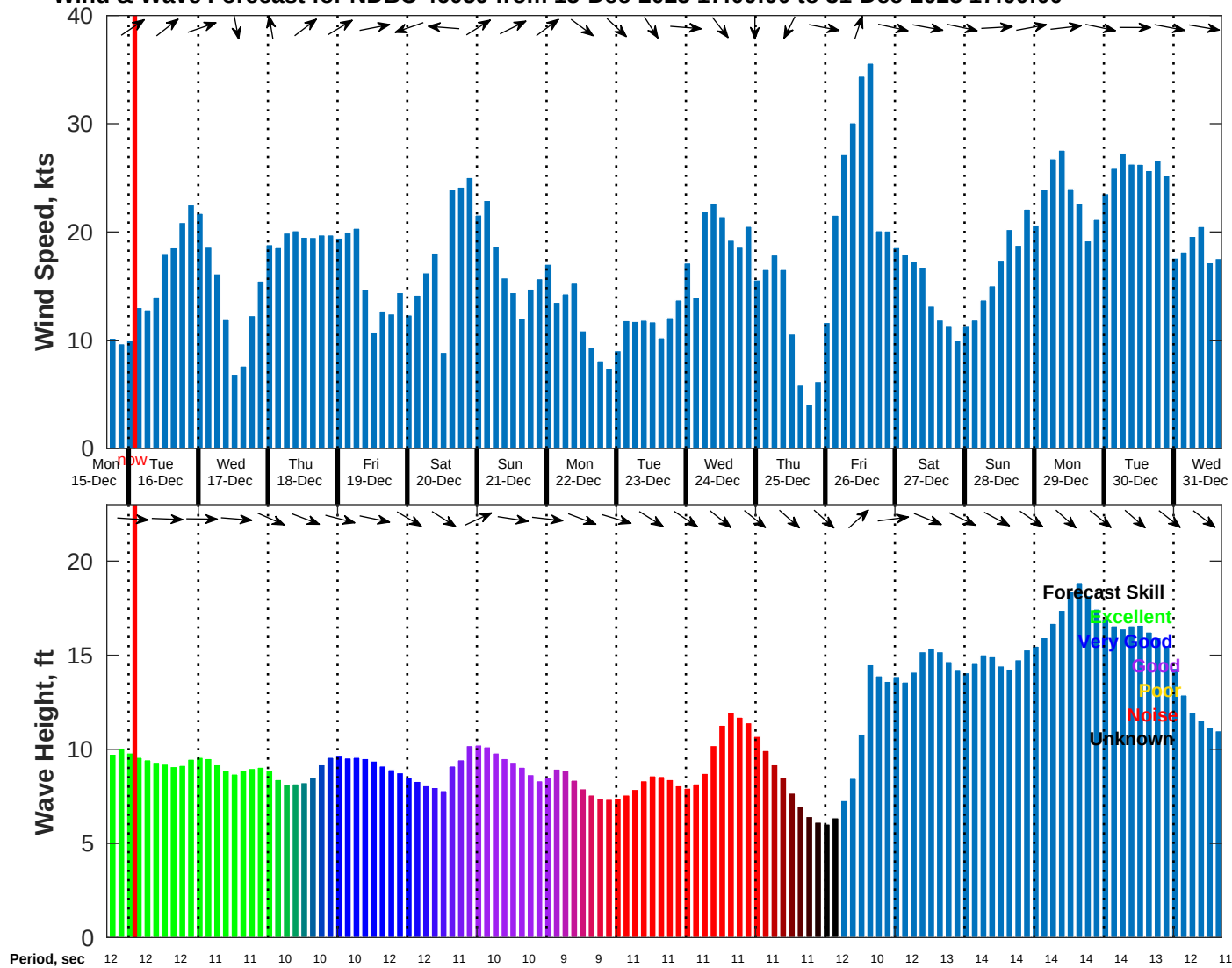
Wind & Wave Forecast for NDBC 46059 from 15-Dec-2025 17:00:00 to 31-Dec-2025 17:00:00
