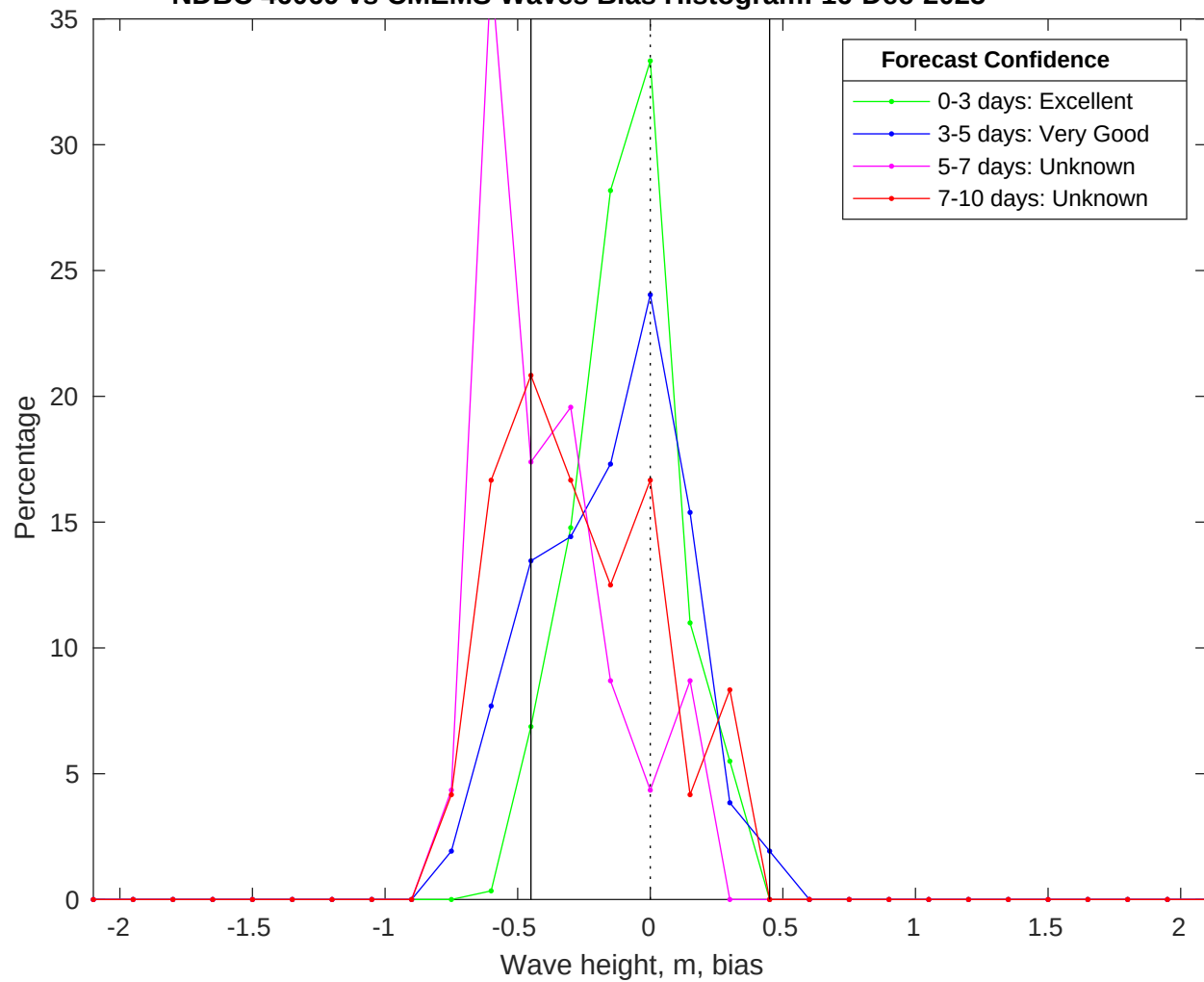
NDBC 46069 vs CMEMS Waves Bias Histogram: 16-Dec-2025
