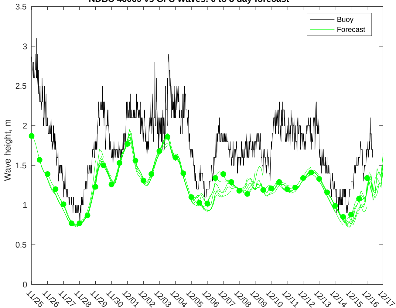
NDBC 46069 vs GFS Waves: 0 to 3 day forecast
