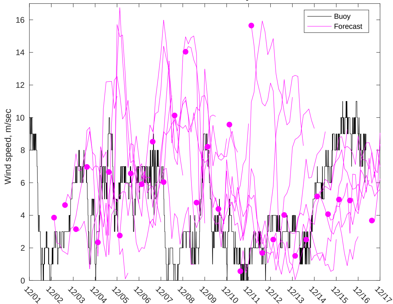
NDBC 46069 vs GFS Winds: 7 to 10 day forecast
