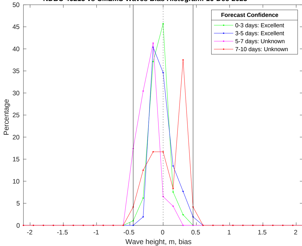
NDBC 46215 vs CMEMS Waves Bias Histogram: 16-Dec-2025
