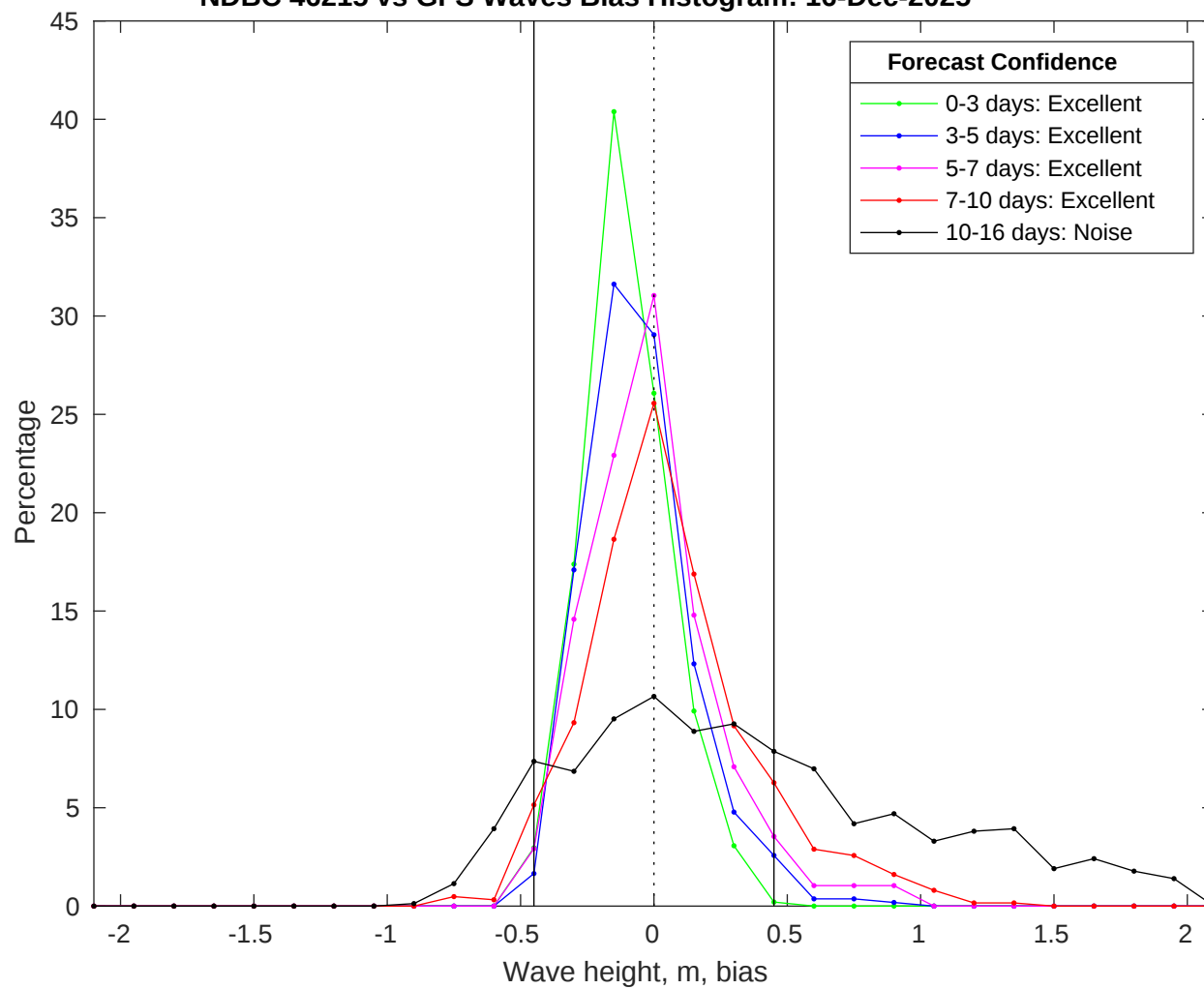
NDBC 46215 vs GFS Waves Bias Histogram: 16-Dec-2025
