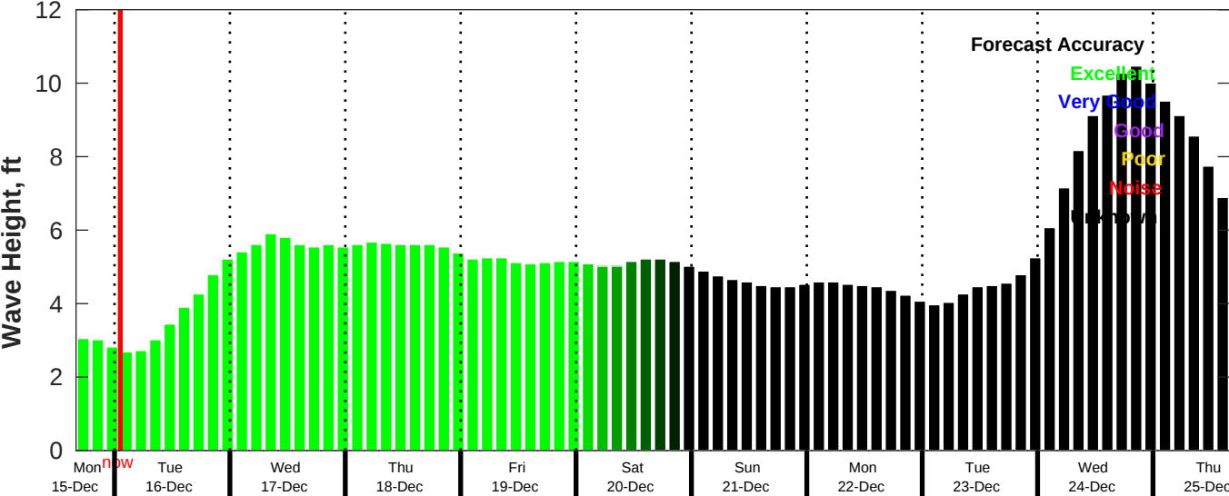
CMEMS Wave Forecast for NDBC 46215 from 15-Dec-2025 16:00:00 to 25-Dec-2025 16:00:00
