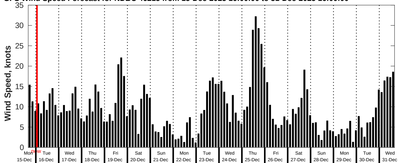
GFS Wind Speed Forecast for NDBC 46215 from 15-Dec-2025 16:00:00 to 31-Dec-2025 16:00:00
