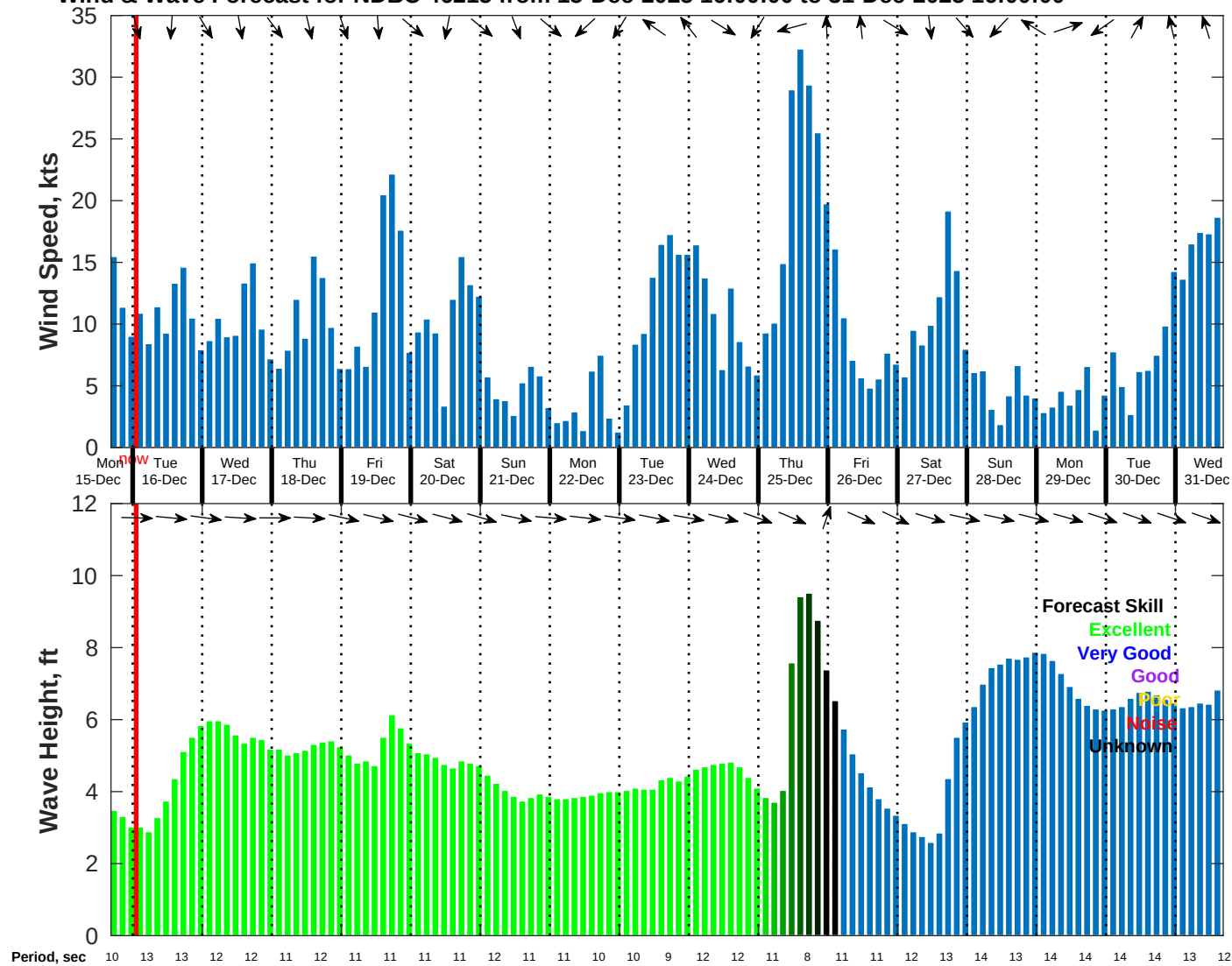
Wind & Wave Forecast for NDBC 46215 from 15-Dec-2025 16:00:00 to 31-Dec-2025 16:00:00
