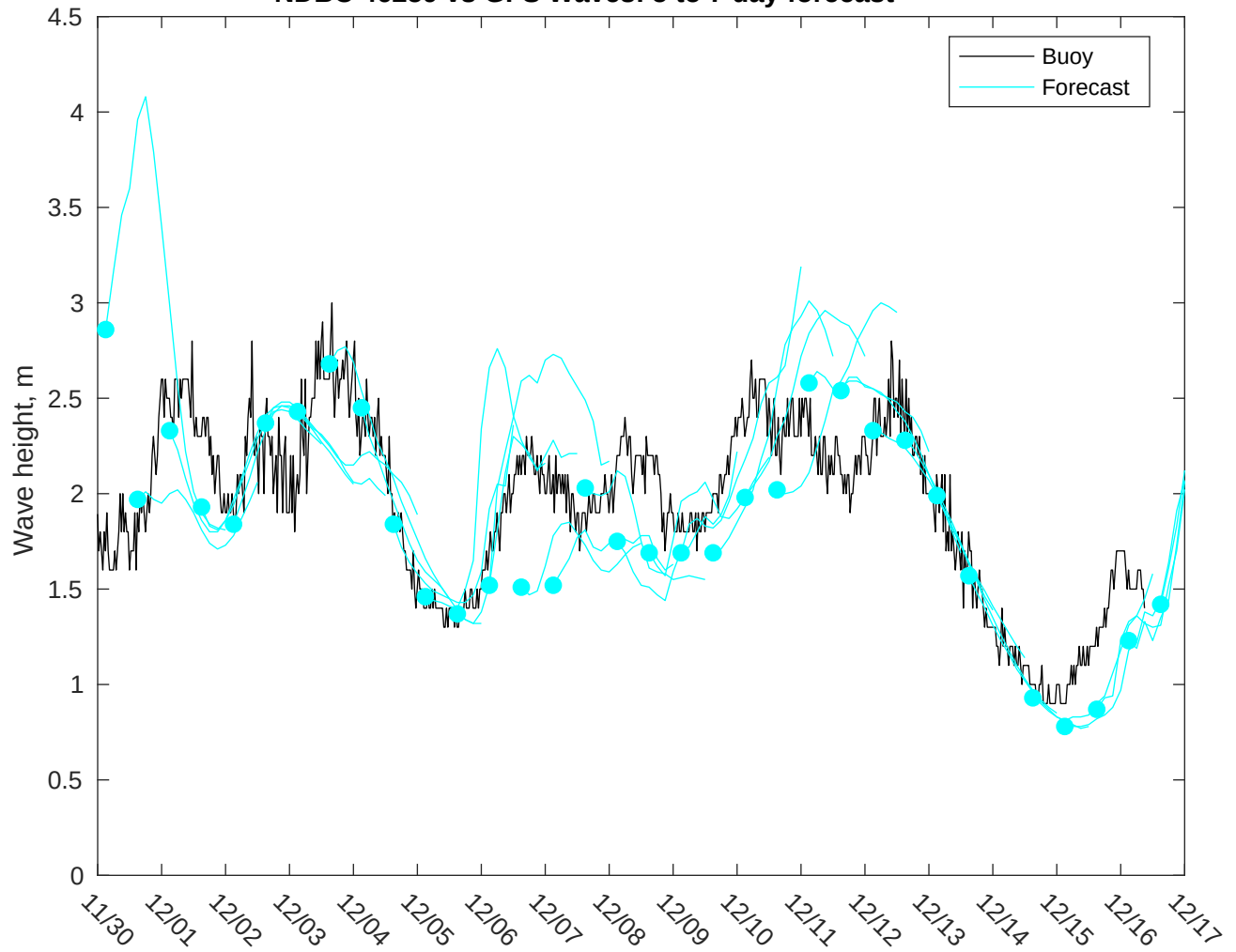
NDBC 46259 vs GFS Waves: 5 to 7 day forecast
