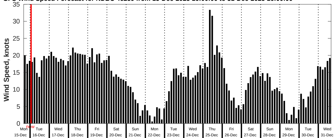
GFS Wind Speed Forecast for NDBC 46259 from 15-Dec-2025 16:00:00 to 31-Dec-2025 16:00:00
