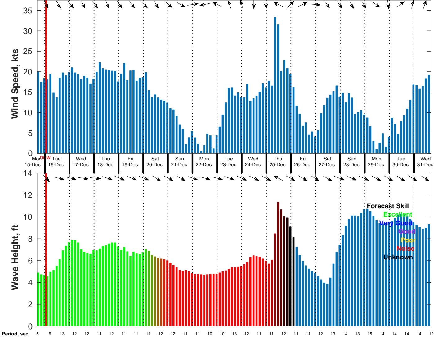
Wind & Wave Forecast for NDBC 46259 from 15-Dec-2025 16:00:00 to 31-Dec-2025 16:00:00
