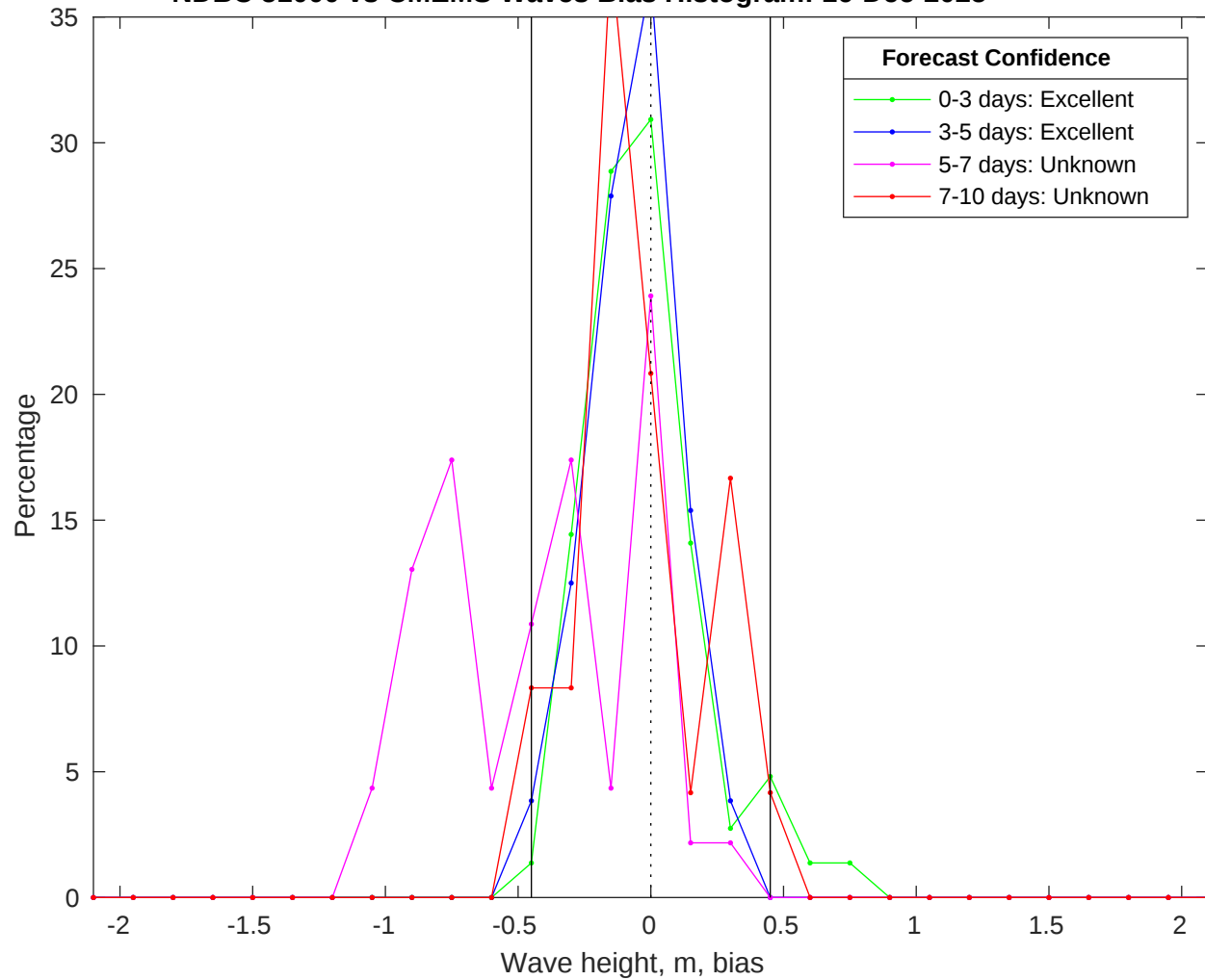
NDBC 51000 vs CMEMS Waves Bias Histogram: 16-Dec-2025
