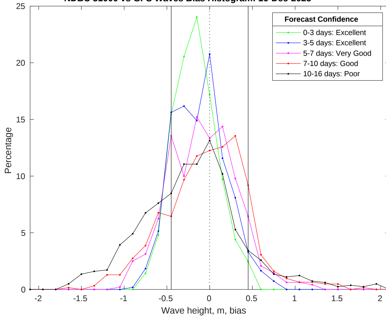
NDBC 51000 vs GFS Waves Bias Histogram: 16-Dec-2025
