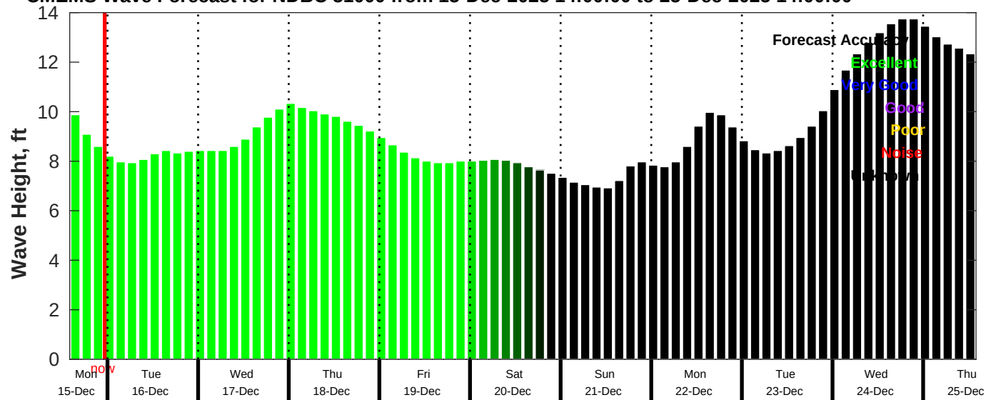
CMEMS Wave Forecast for NDBC 51000 from 15-Dec-2025 14:00:00 to 25-Dec-2025 14:00:00
