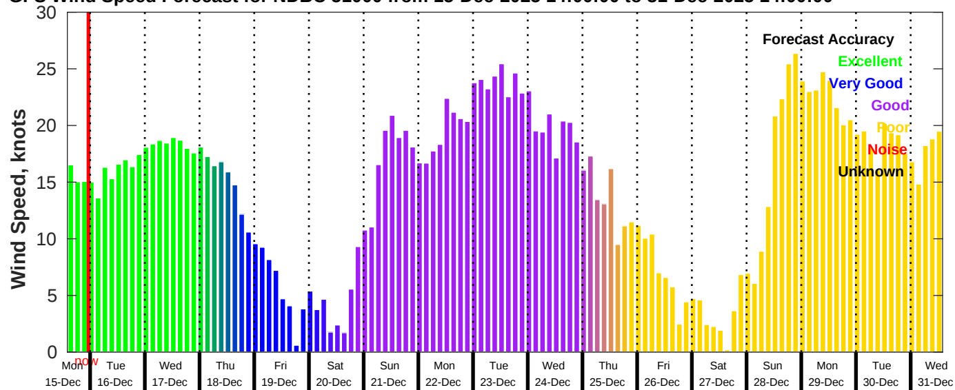
GFS Wind Speed Forecast for NDBC 51000 from 15-Dec-2025 14:00:00 to 31-Dec-2025 14:00:00
