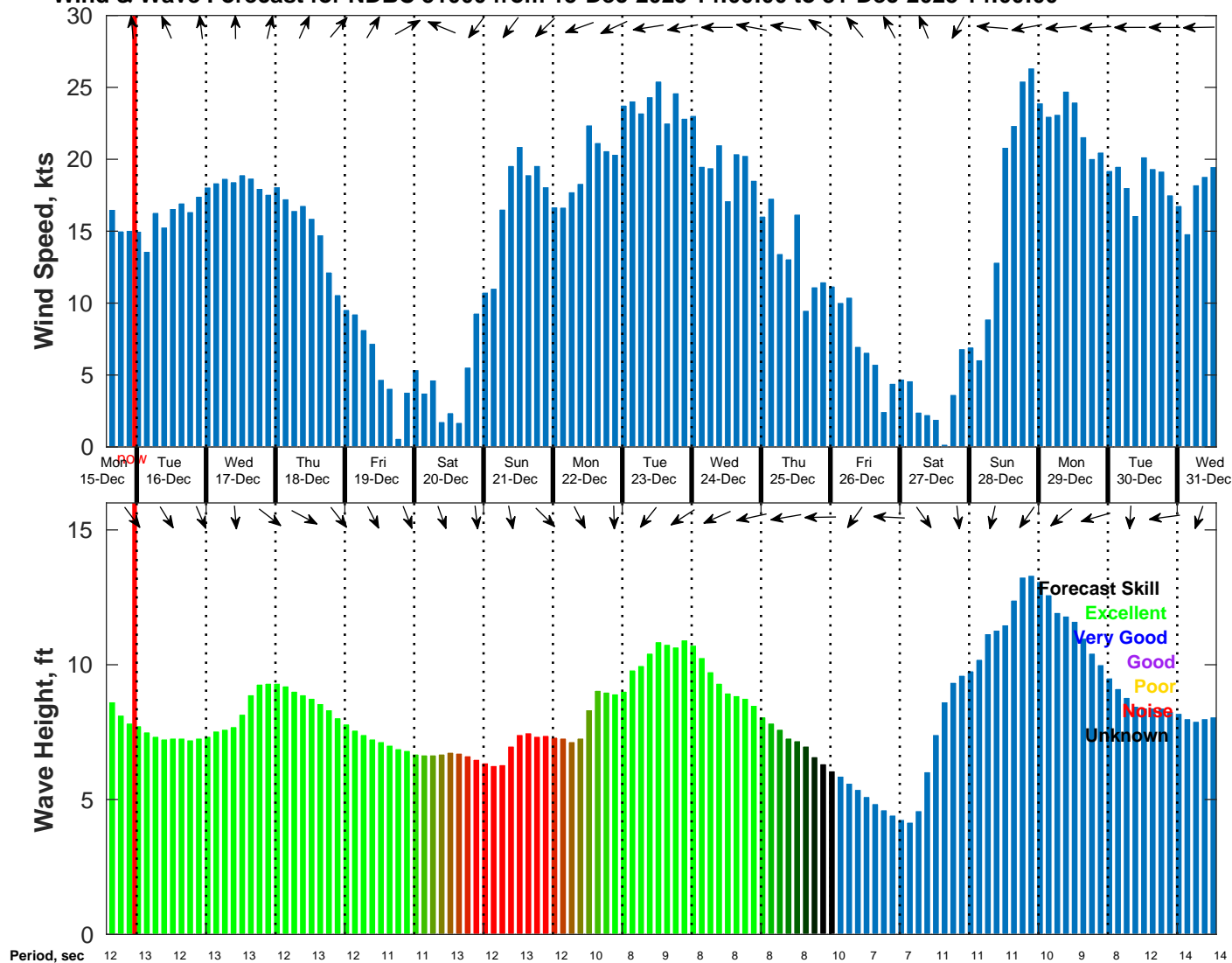
Wind & Wave Forecast for NDBC 51000 from 15-Dec-2025 14:00:00 to 31-Dec-2025 14:00:00
