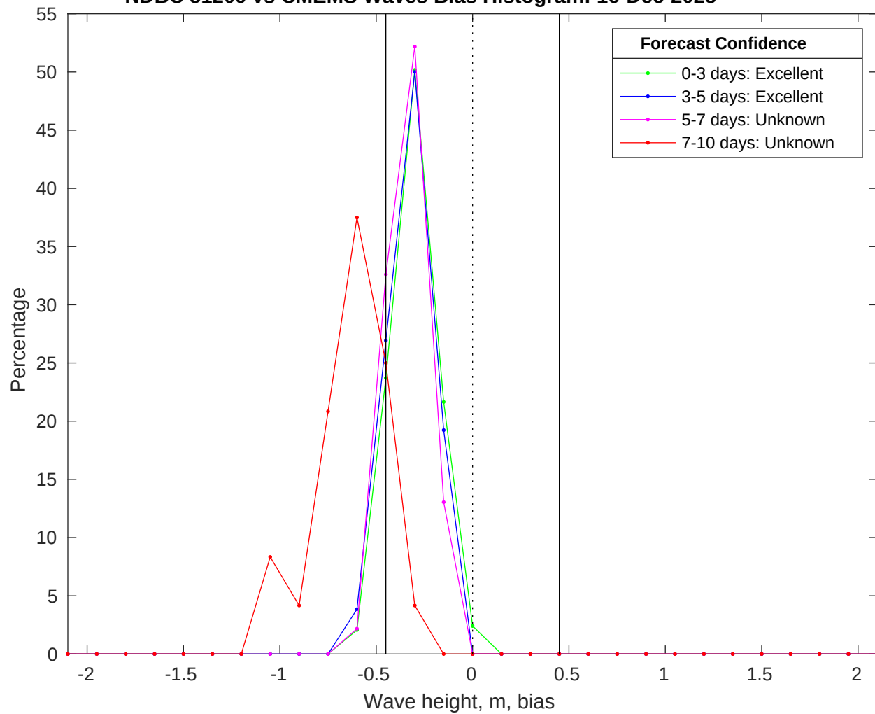
NDBC 51209 vs CMEMS Waves Bias Histogram: 16-Dec-2025
