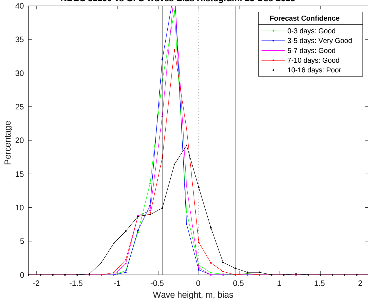
NDBC 51209 vs GFS Waves Bias Histogram: 16-Dec-2025
