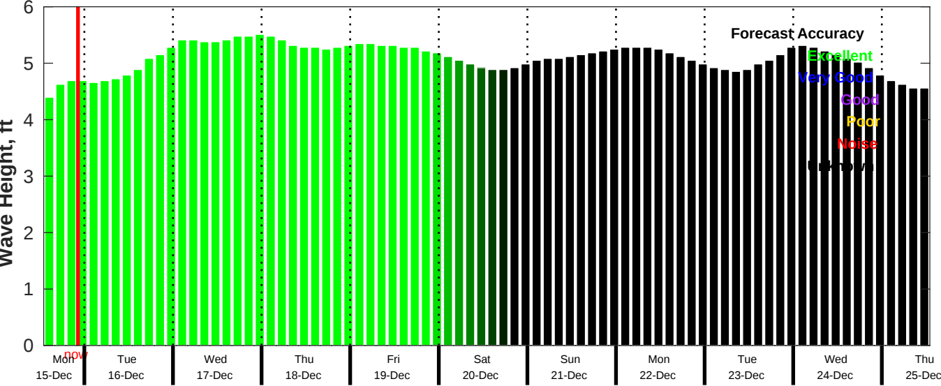
CMEMS Wave Forecast for NDBC 51209 from 15-Dec-2025 13:00:00 to 25-Dec-2025 13:00:00
