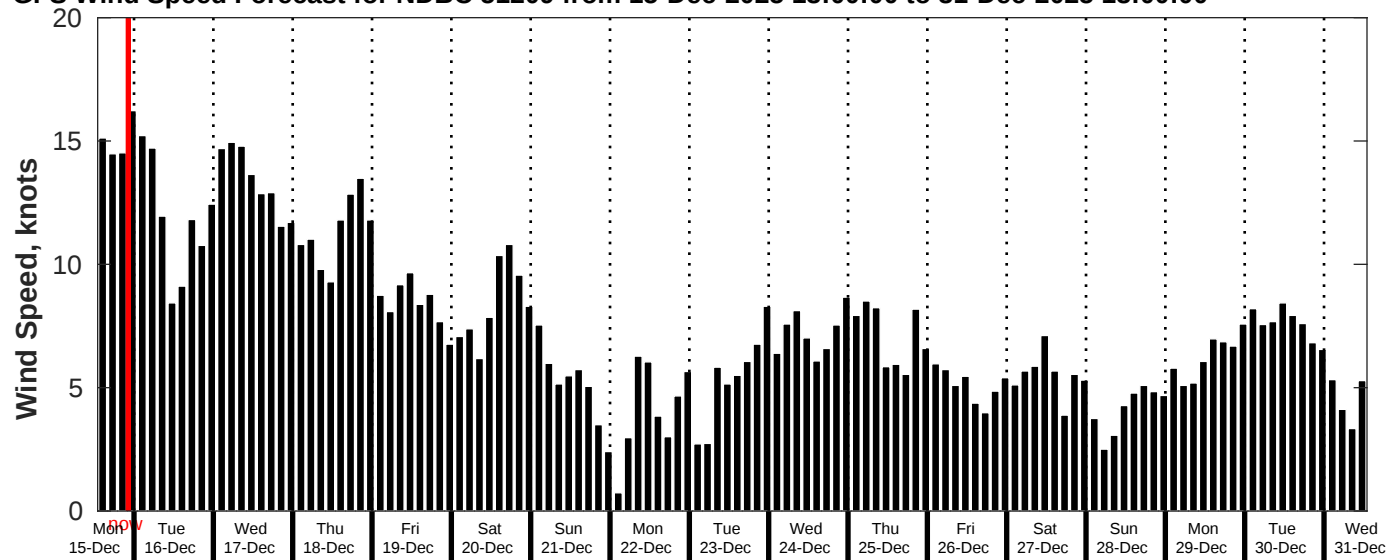
GFS Wind Speed Forecast for NDBC 51209 from 15-Dec-2025 13:00:00 to 31-Dec-2025 13:00:00
