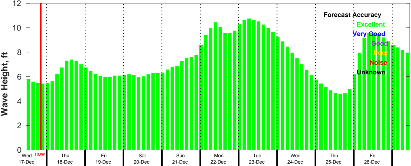
CMEMS Wave Forecast for NDBC 52211 from 16-Dec-2025 11:00:00 to 26-Dec-2025 11:00:00
