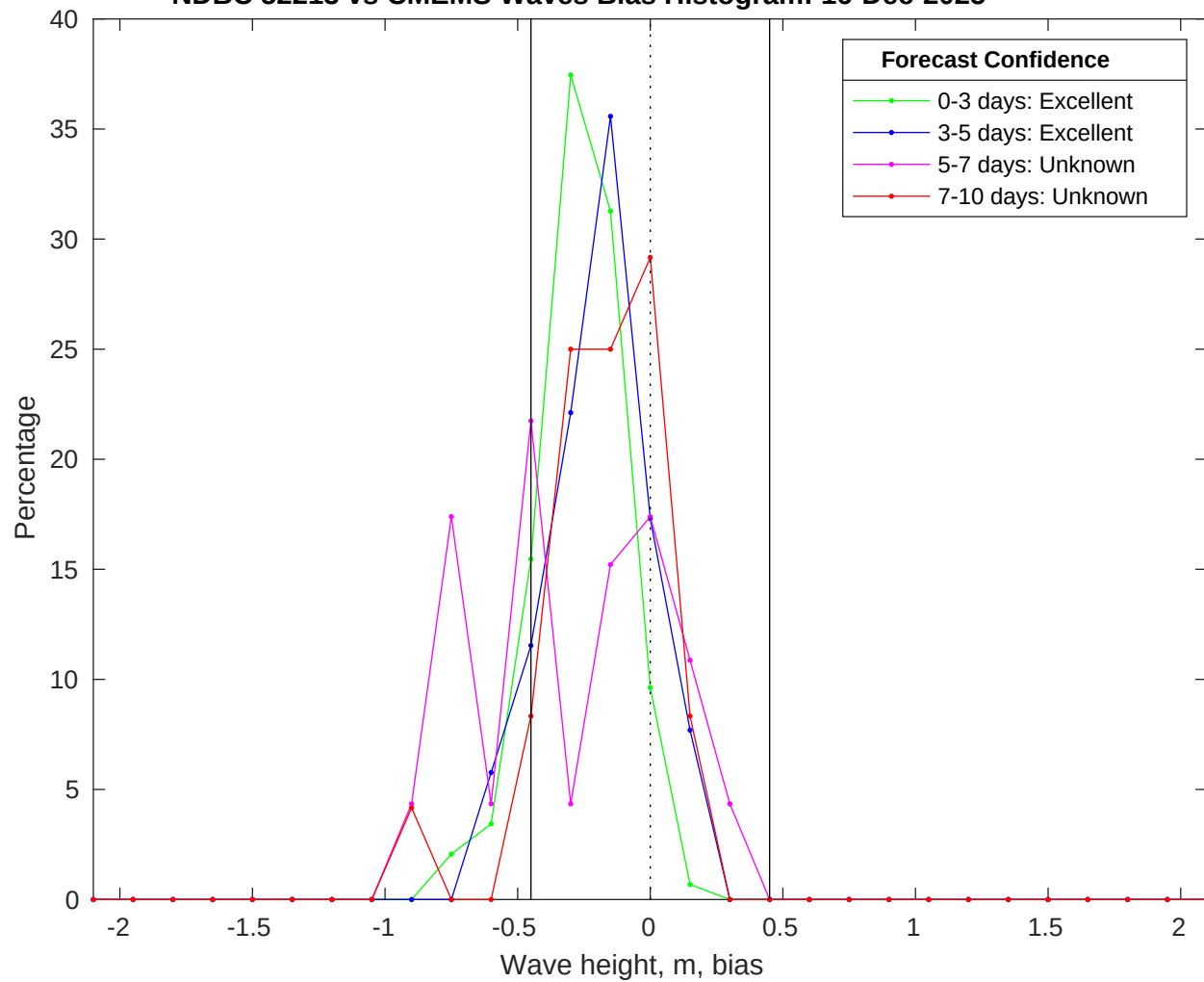
NDBC 52213 vs CMEMS Waves Bias Histogram: 16-Dec-2025
