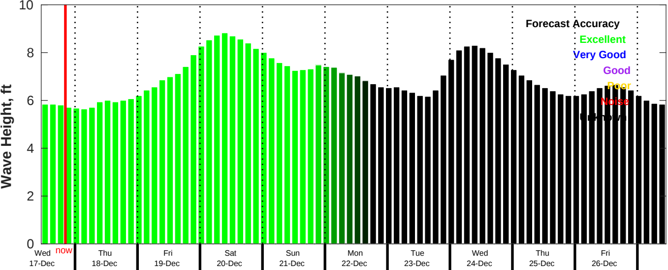
CMEMS Wave Forecast for NDBC 52213 from 16-Dec-2025 11:00:00 to 26-Dec-2025 11:00:00
