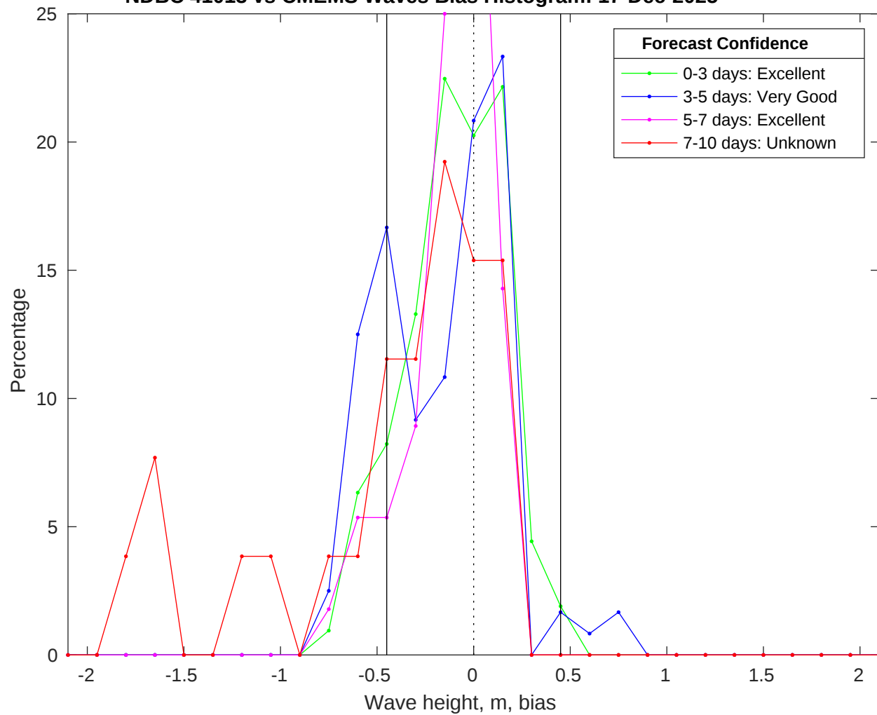
NDBC 41013 vs CMEMS Waves Bias Histogram: 17-Dec-2025
