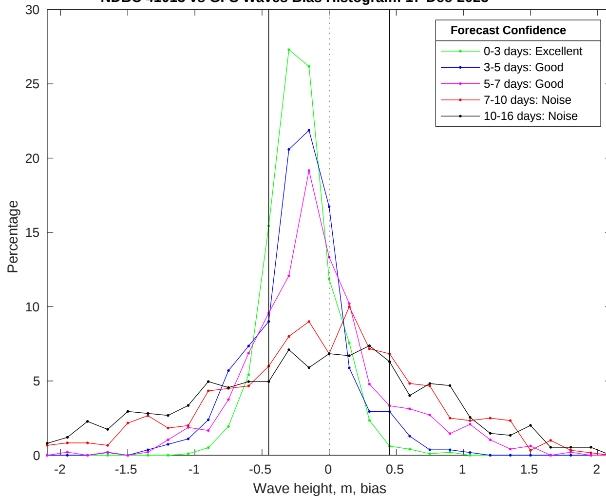
NDBC 41013 vs GFS Waves Bias Histogram: 17-Dec-2025
