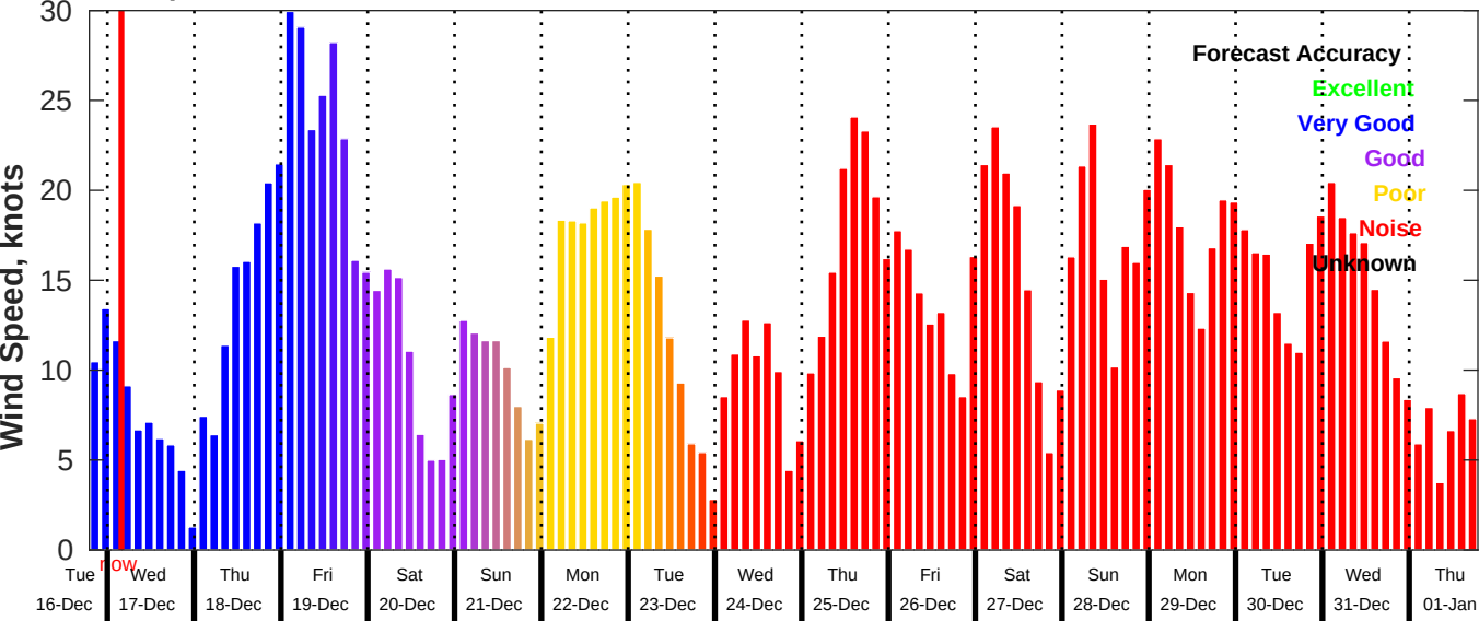
GFS Wind Speed Forecast for NDBC 41013 from 16-Dec-2025 19:00:00 to 01-Jan-2026 19:00:00
