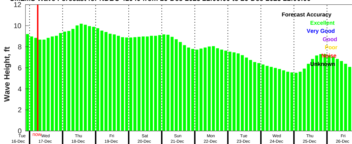
CMEMS Wave Forecast for NDBC 41040 from 16-Dec-2025 21:00:00 to 26-Dec-2025 21:00:00
