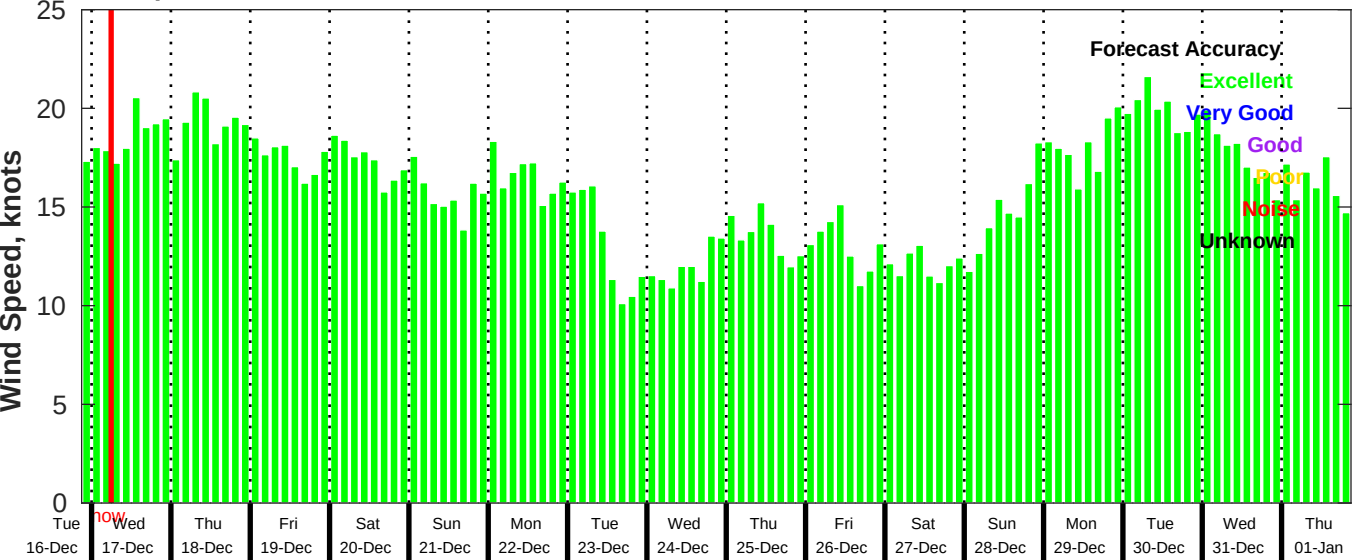
GFS Wind Speed Forecast for NDBC 41040 from 16-Dec-2025 21:00:00 to 01-Jan-2026 21:00:00
