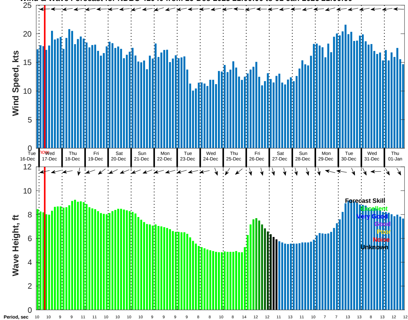
Wind & Wave Forecast for NDBC 41040 from 16-Dec-2025 21:00:00 to 01-Jan-2026 21:00:00
