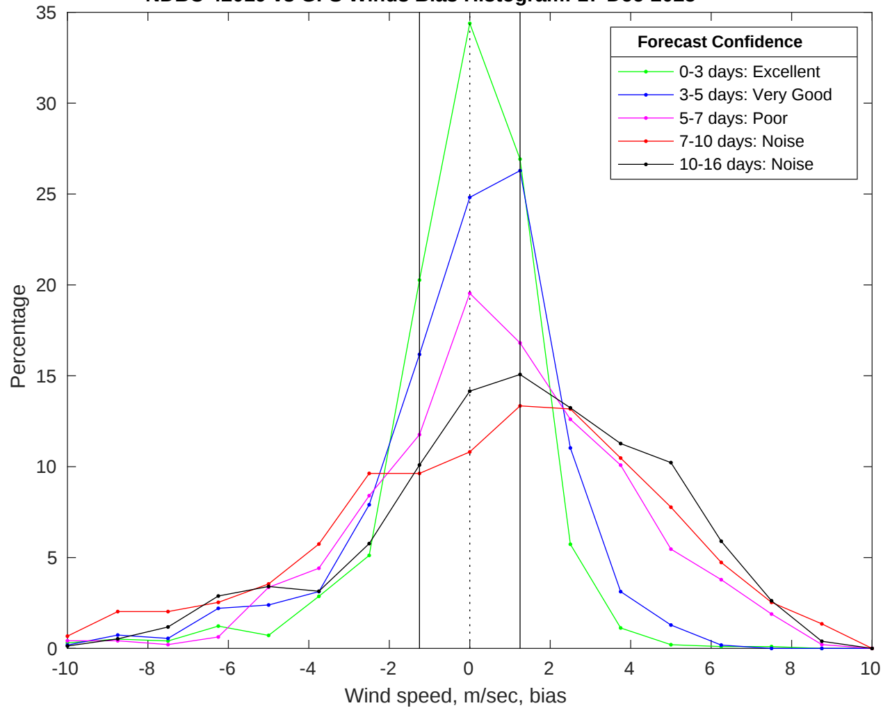
NDBC 42019 vs GFS Winds Bias Histogram: 17-Dec-2025
