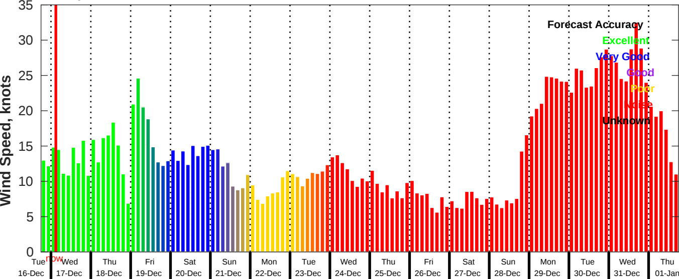
GFS Wind Speed Forecast for NDBC 42019 from 16-Dec-2025 18:00:00 to 01-Jan-2026 18:00:00
