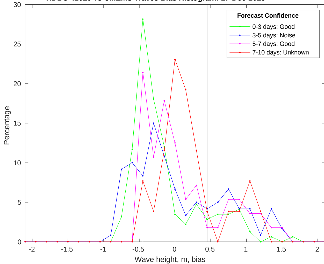
NDBC 42020 vs CMEMS Waves Bias Histogram: 17-Dec-2025
