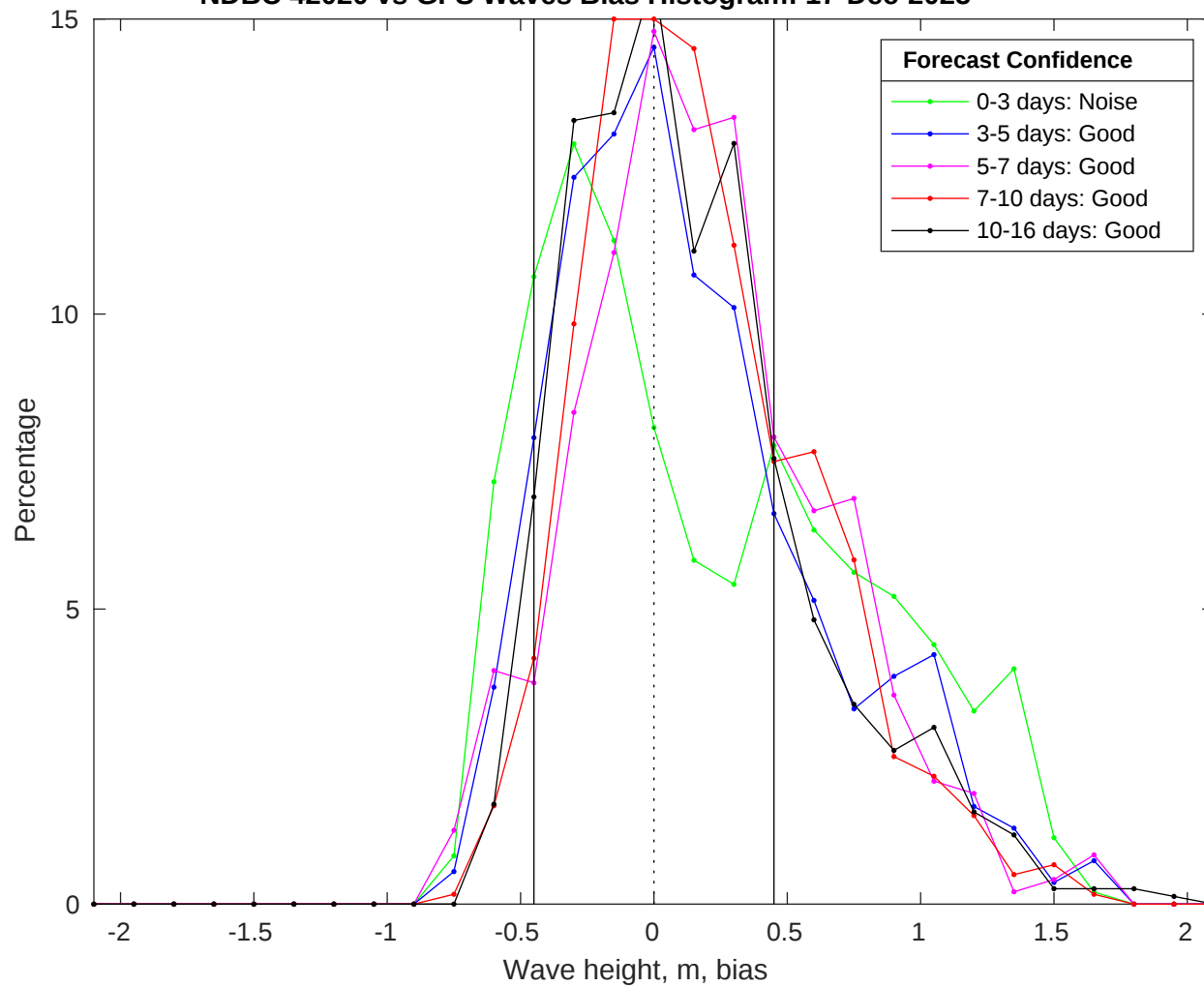
NDBC 42020 vs GFS Waves Bias Histogram: 17-Dec-2025
