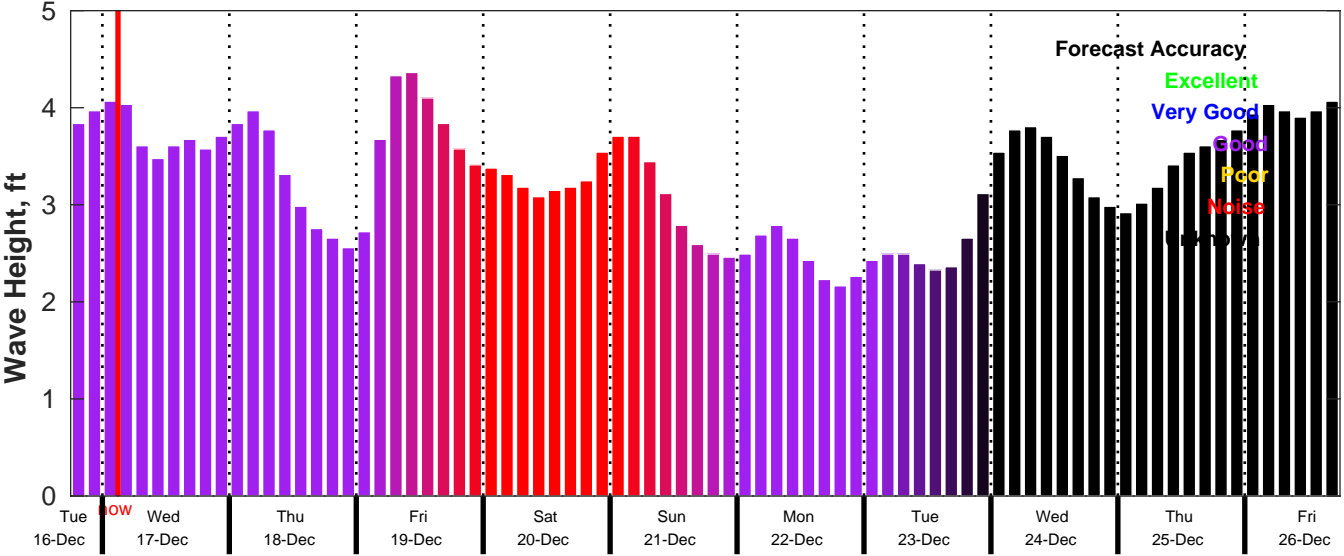
CMEMS Wave Forecast for NDBC 42020 from 16-Dec-2025 18:00:00 to 26-Dec-2025 18:00:00
