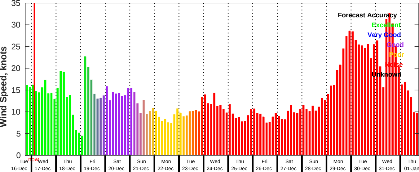
GFS Wind Speed Forecast for NDBC 42020 from 16-Dec-2025 18:00:00 to 01-Jan-2026 18:00:00
