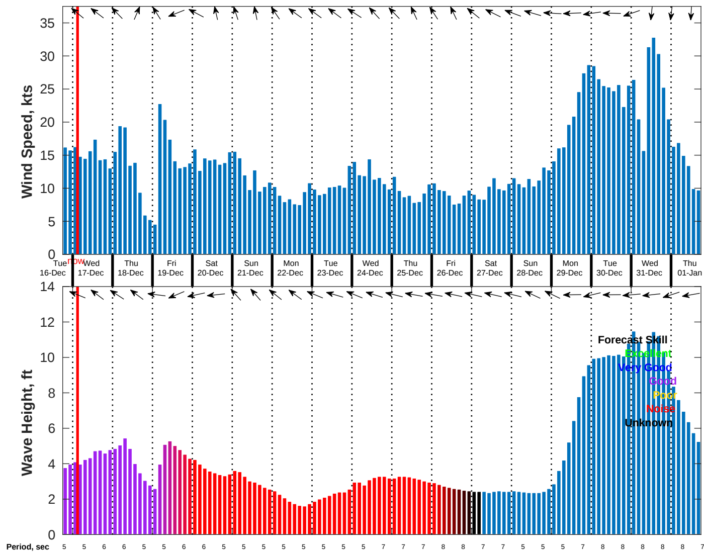
Wind & Wave Forecast for NDBC 42020 from 16-Dec-2025 18:00:00 to 01-Jan-2026 18:00:00
