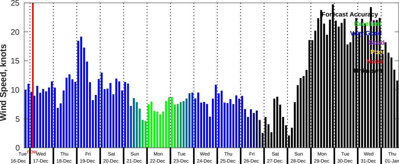
GFS Wind Speed Forecast for NDBC 42035 from 16-Dec-2025 18:00:00 to 01-Jan-2026 18:00:00
