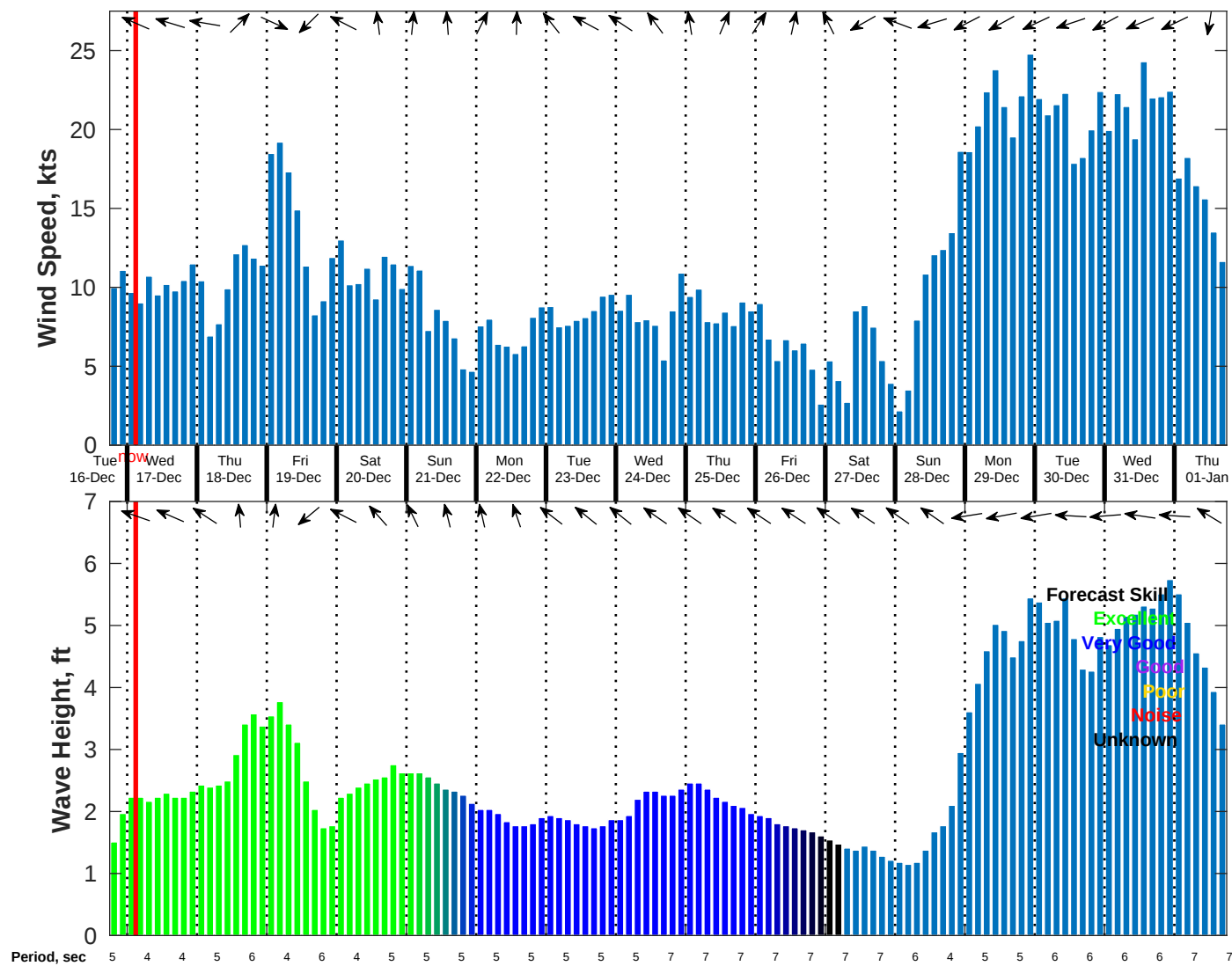
Wind & Wave Forecast for NDBC 42035 from 16-Dec-2025 18:00:00 to 01-Jan-2026 18:00:00
