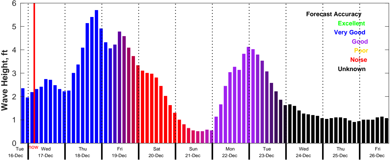
CMEMS Wave Forecast for NDBC 42036 from 16-Dec-2025 19:00:00 to 26-Dec-2025 19:00:00
