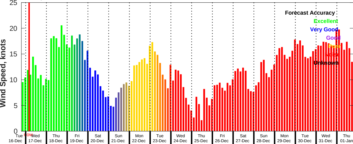
GFS Wind Speed Forecast for NDBC 42036 from 16-Dec-2025 19:00:00 to 01-Jan-2026 19:00:00
